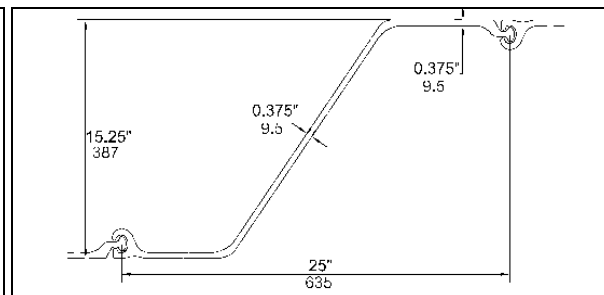
Figure 5: PZC Sheet pile (Type PZC 18) with „Ball and Socket“ interlocking
