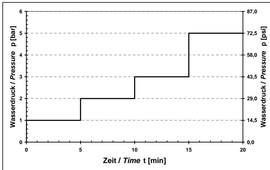
Figure 9: Intended pressure control
