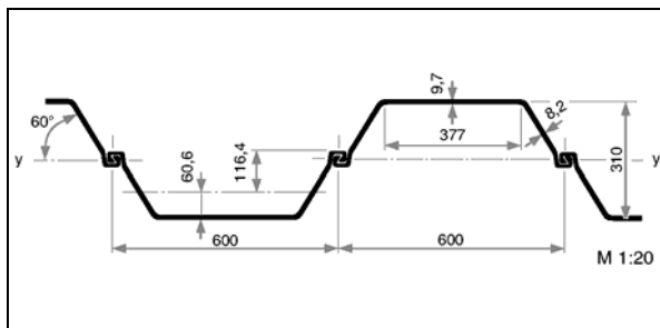
Figure 4: LARSEN-Sheet pile (Type 603) with interlocking type 1 according to [3]
